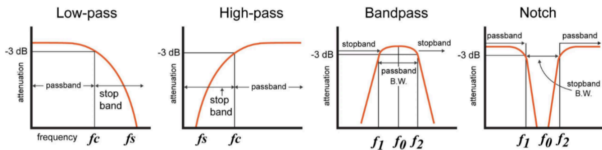
Frequency Domain Filters in 1D
